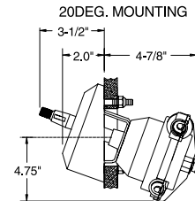
MOUNTING OPTIONS STARBOARD SIDE VIEW 20DEG. MOUNTING
