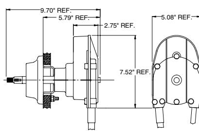
SYSTEM OPTIONS 4.2 NFB SINGLE HELM & CABLE ( SH 4910 ) TOP VIEW
