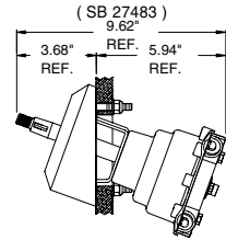
MOUNTING OPTIONS STARBOARD SIDE VIEW 20DEG. BEZEL MOUNTING ( SB 27483 )
