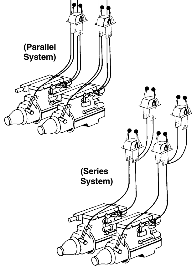
SINGLE FUNCTION CONTROL, TWIN ENGINE, TWIN STATION
